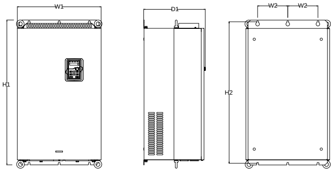
图 B-6 132G/160P~200G/220P 壁挂安装
