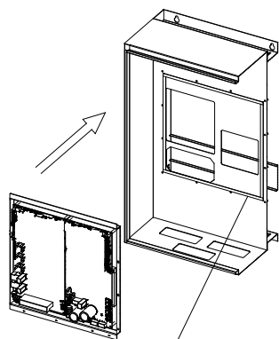
柜体与整机安装面之间加防水胶条
